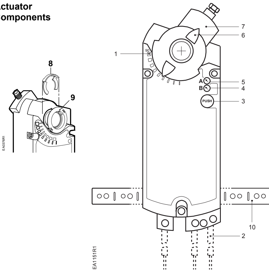
Figure 11. Components of the 3-Position Actuator.
