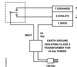
Figure 22. 24 Vac, 3-Position Control.
