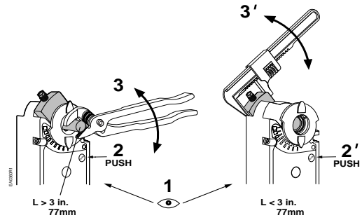
Figure 14. Manual Override.
