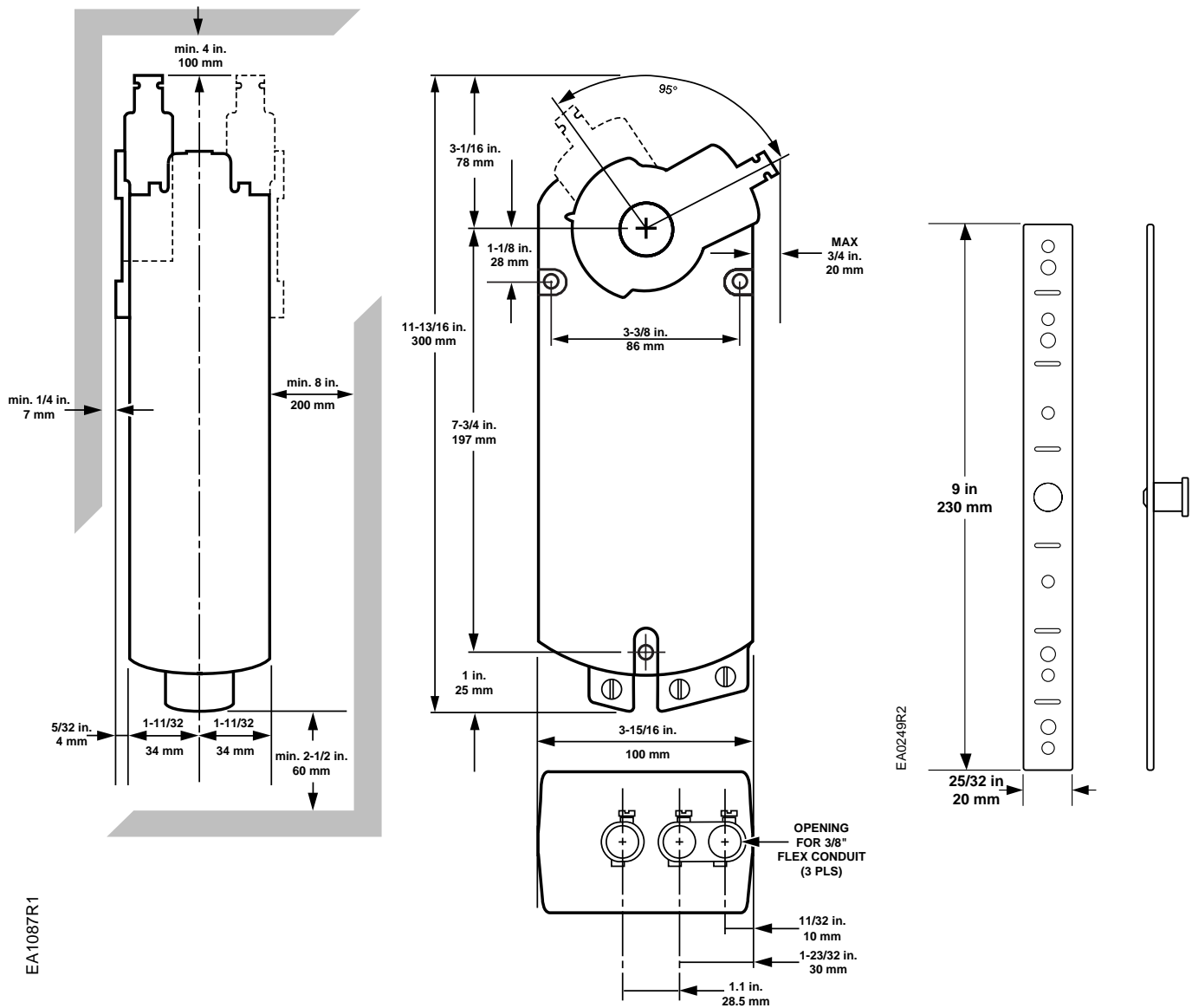
Figure 24. Dimensions of the GBB/GIB Actuator and Mounting Bracket in Inches (Millimeters).
